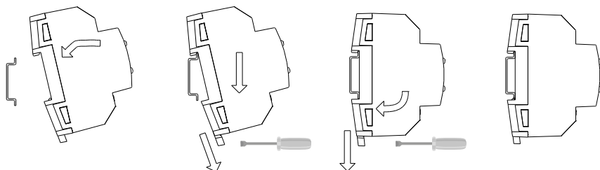
Attaching ShutterBOX Drive 4CH to DIN rail:
