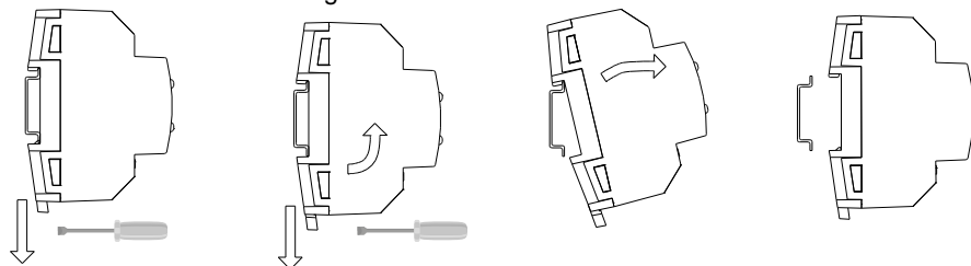
Removing ShutterBOX Drive 4CH from DIN rail:
