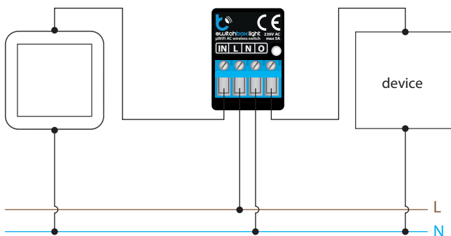
CONNECTION DIAGRAM
