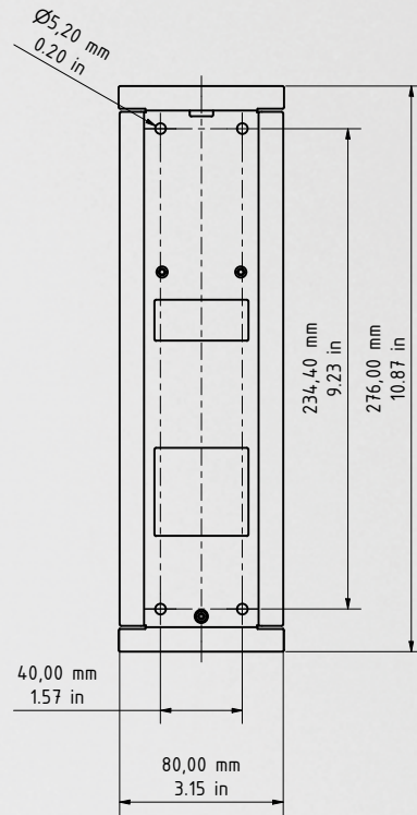
Flush-mounting housing (backbox)
