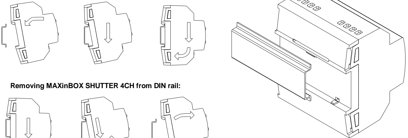
Figure 3. Mounting MAXinBOX SHUTTER 4CH on a DIN rail
