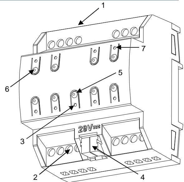
Figure 1. MAXinBOX SHUTTER 4CH
