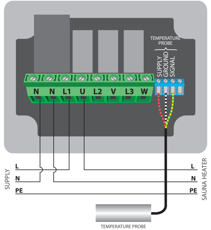
SINGLE PHASE SUPPLY, SINGLE PHASE HEATER
