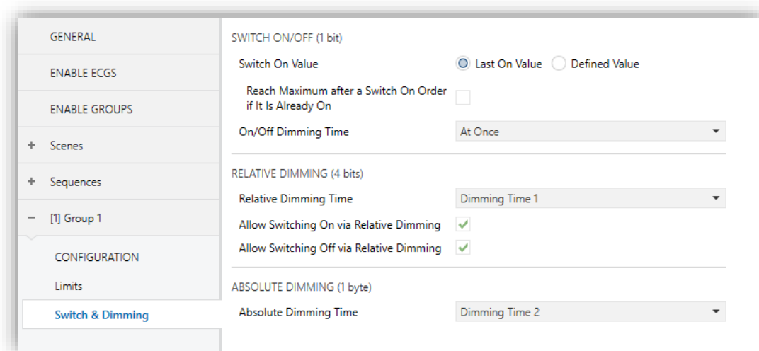
Figure 25. Switch & Dimming
